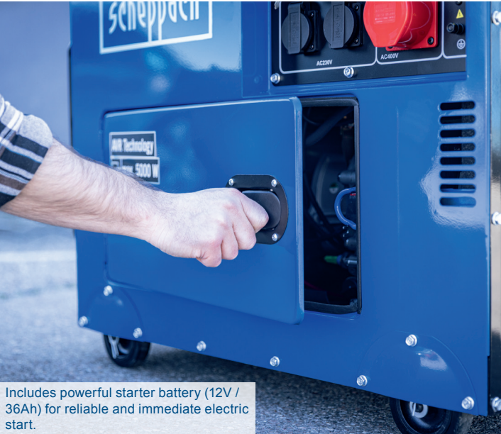
Integrated electric start with ignition lock for convenient and safe starting of the unit.
